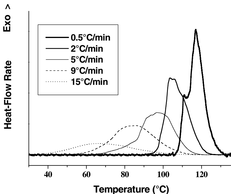
Figure 1. DSC thermograms of PHB powder crystallized at various cooling rates after melting at 193°C for 3 min. Measurements performed with Perkin-Elmer Pyris 1 DSC.
