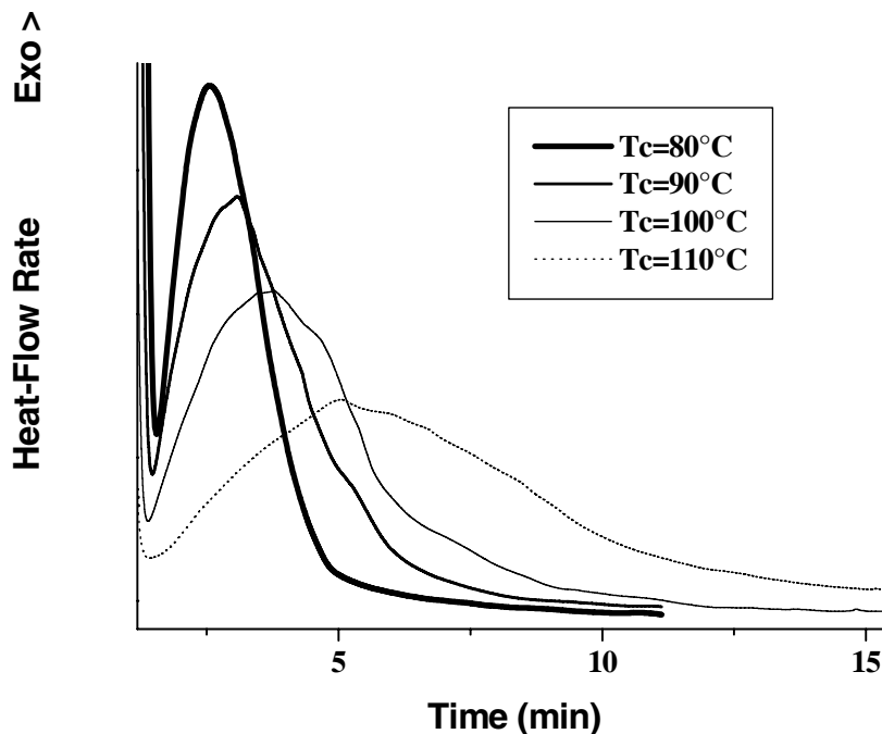
Figure 2. DSC thermograms of PHB powder during isothermal crystallization at 80 and 100°C, after melting at 193°C for 3 min. Measurements performed with Perkin-Elmer Pyris 1 DSC.
