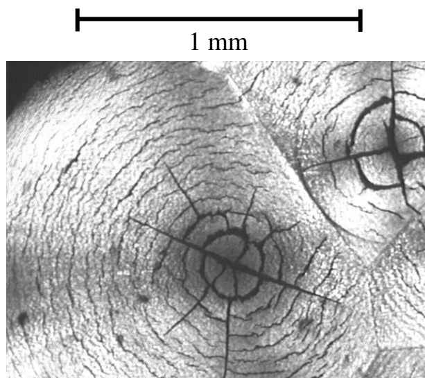
Figure 3. Optical micrograph (crossed polars) of PHB film, crystallized during cooling at 5°C/min, after melting at 200°C for 3 min.
