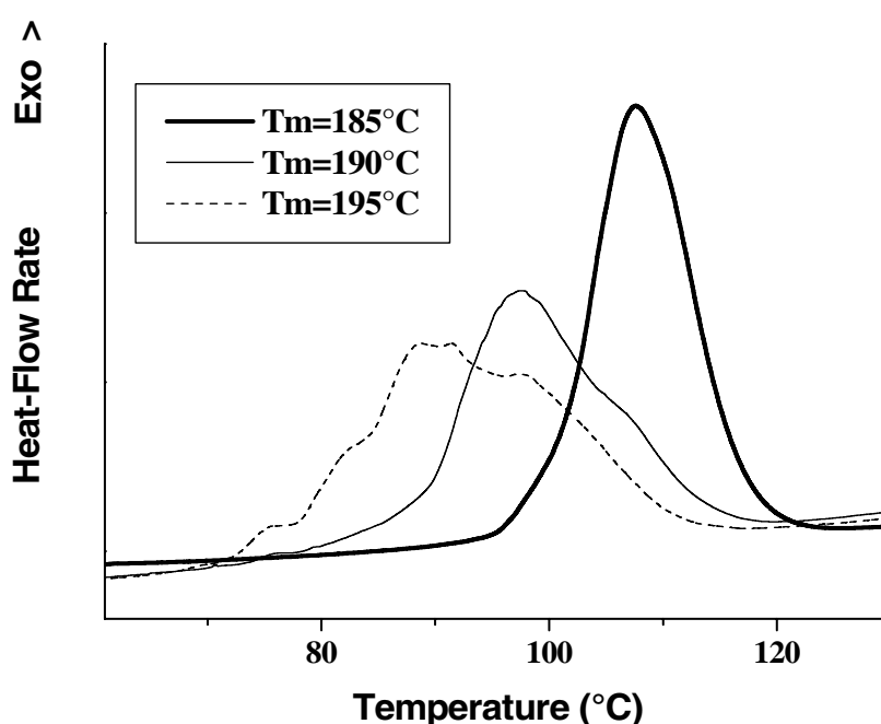
Figure 4. DSC thermograms of PHB film, measured during crystallization at 5°C/min, after melting for 3 min at the indicated temperatures. Measurements performed with Mettler DSC-30.
